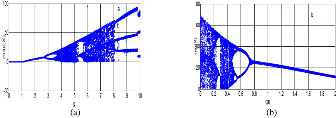
Fig.2. Bifurcation diagram reel circuit : (a). As a function of the parameter g^* , (b) as a function of the parameter Q_0 .
