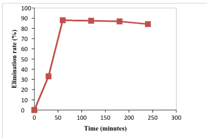
Fig. 3. Effect of contact time on the removal of ions lead on activated carbon.
