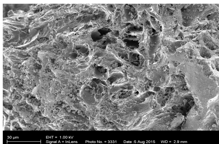
Fig. 1. High magnification FESEM micrograph of activated carbon.
