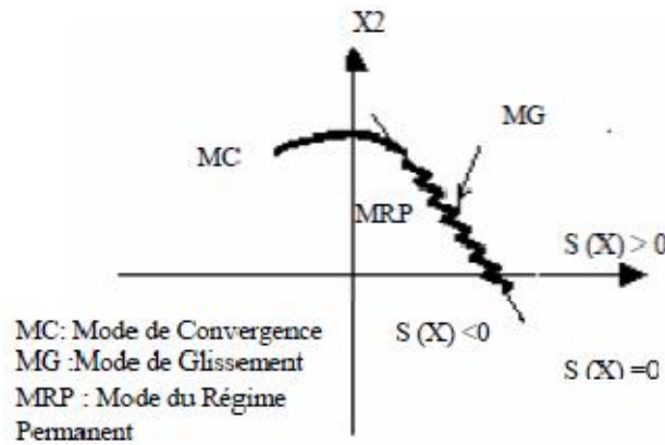
Fig. 2: Modes of trajectory in the plan of phase.
