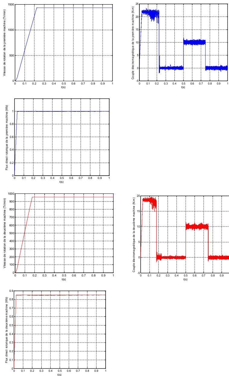
Fig.4: Simulation results of the Sliding mode control of a Five-Phase Series-Connected Two-Motor Drive
