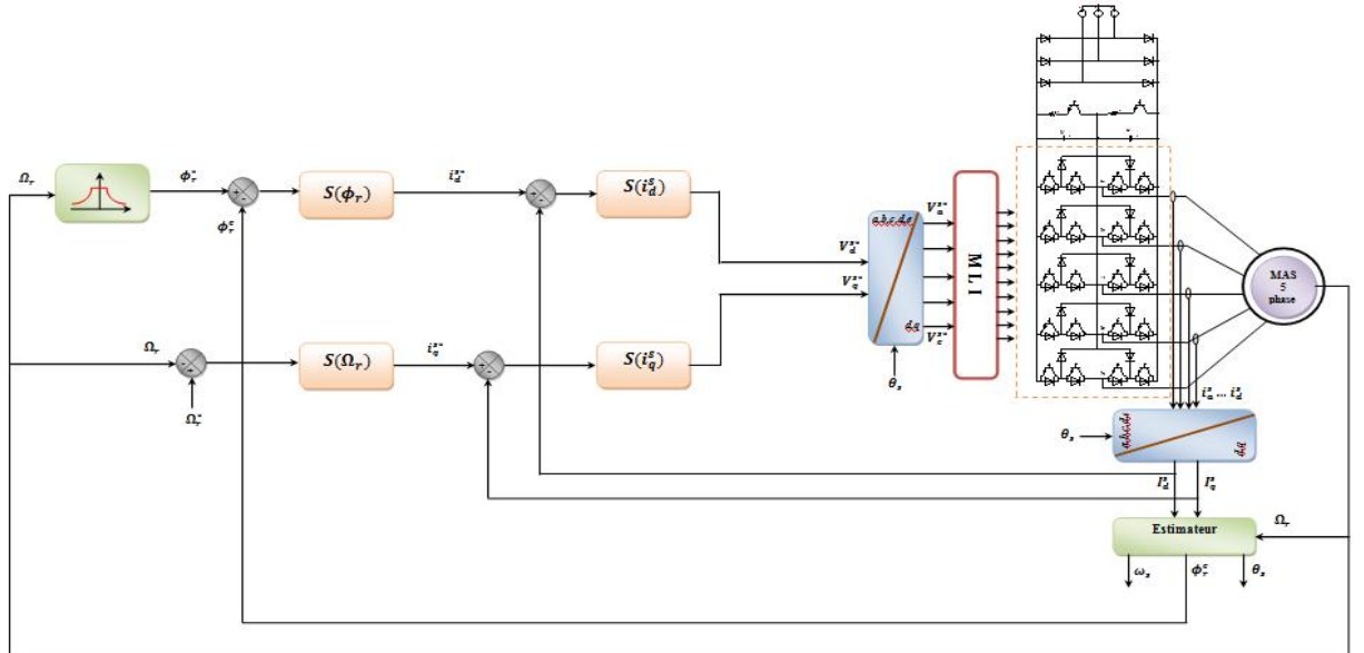
Fig .3: Sliding mode control of a Five-Phase Series-Connected Two-Motor Drive
