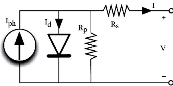
Fig. 1: Solar cell single-diode model
