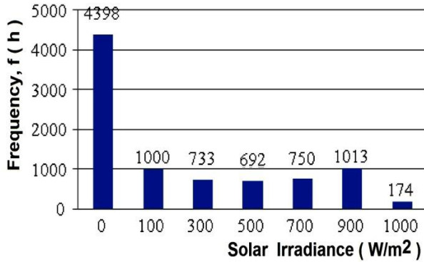
Fig. 3: Solar data frequency histogram (Adrar)
