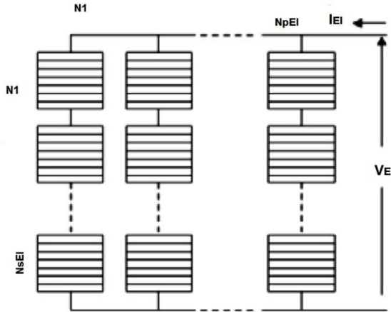
Fig. 2: Block diagram of PEM electrolyser
