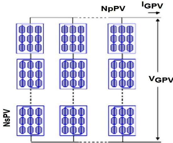
Fig. 1: Synoptic diagram of a PV generator
