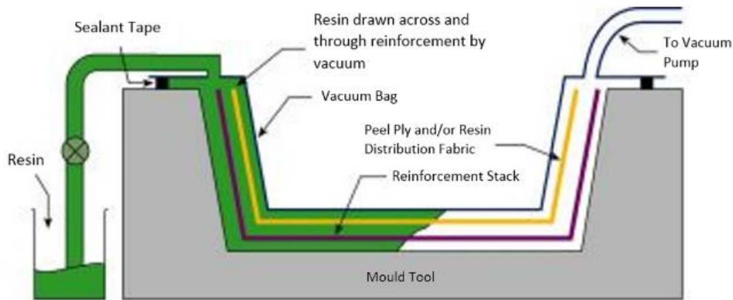
Fig 2. Vacuum infusion proces (Gent, 2014).
