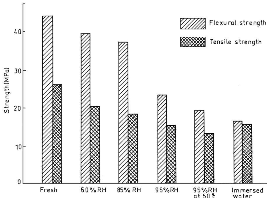
Fig. 1. The effect of humid conditions on strengths of a jute composite (Singh, 2000).
