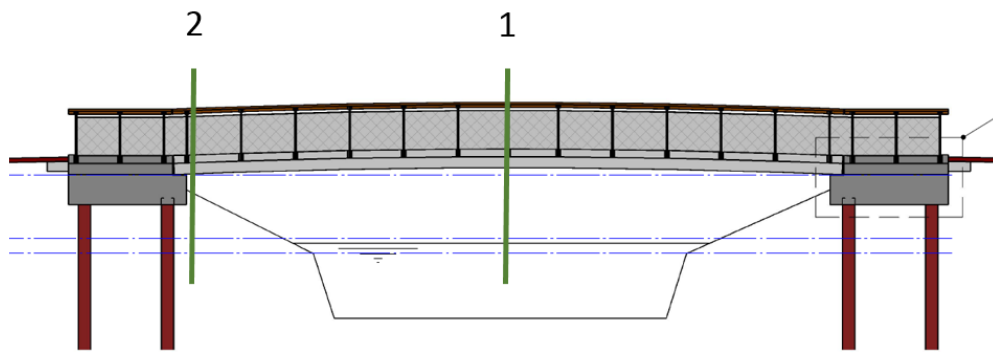
Fig 4. Positions in deck (heester, 2015).
