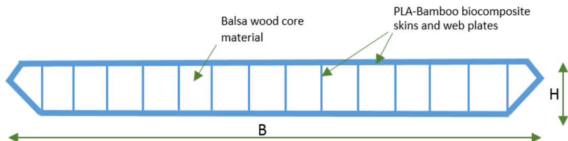
Fig 3. Cross section deck. Where: B=4500mm, H=460mm.
